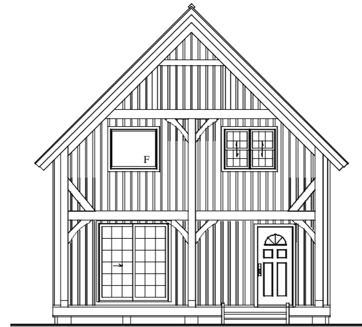
ELEVATION FRONT
