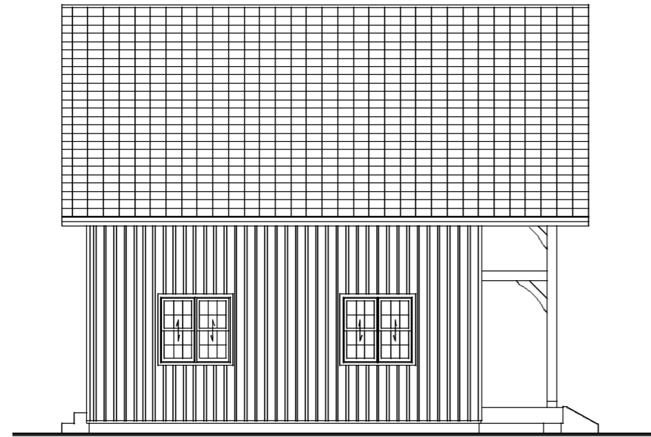
ELEVATION LEFT SIDE
